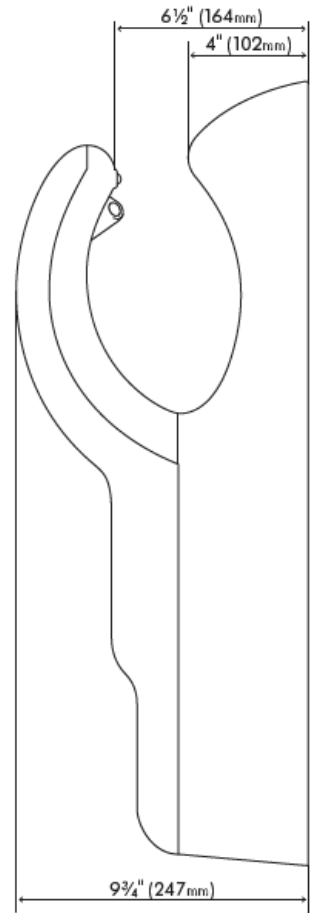
SIDE ELEVATION
