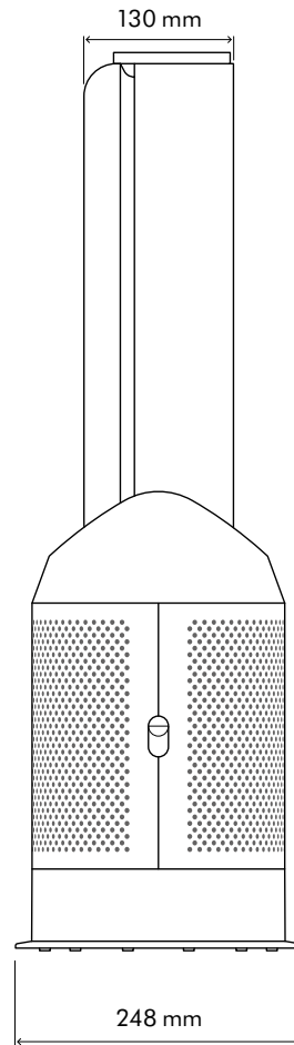
SIDE VIEW
