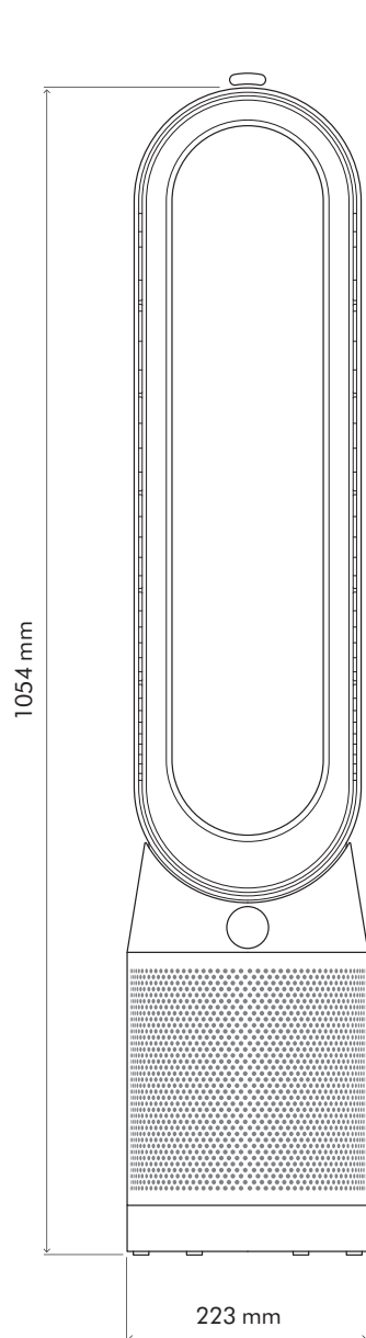
FRONT VIEW
