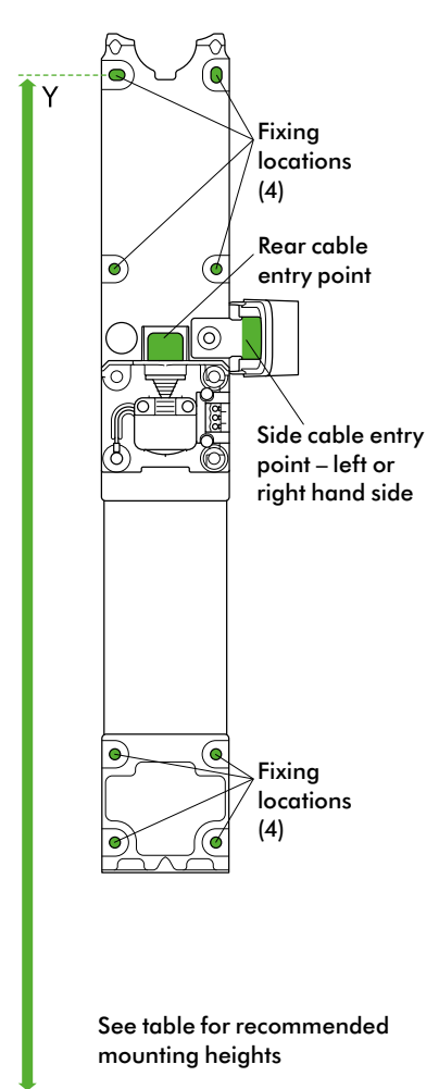
Back plate
