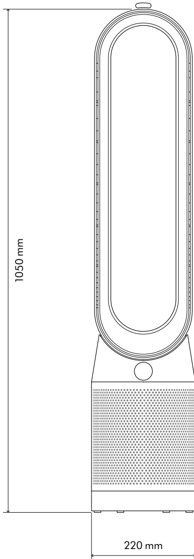
Plan elevation
