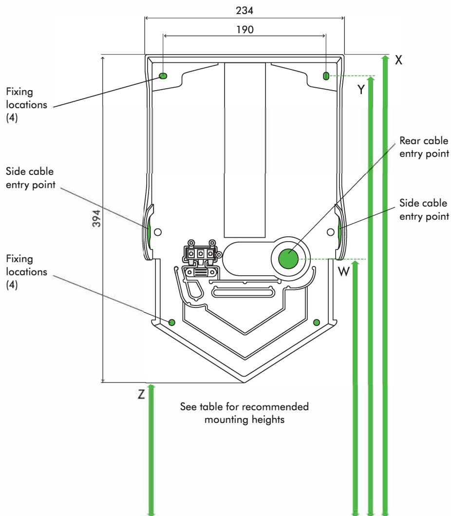
REAR ELEVATION
